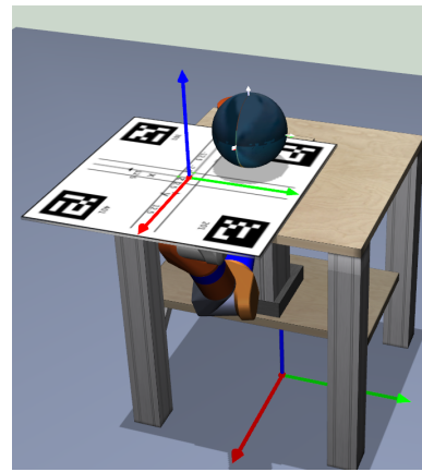
Figure 2.3.: All coordinate frames of the BoP system
