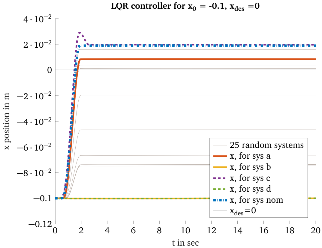
Figure 6.1.: Rcs simulation of LQR controller as designed in Section 4.6
