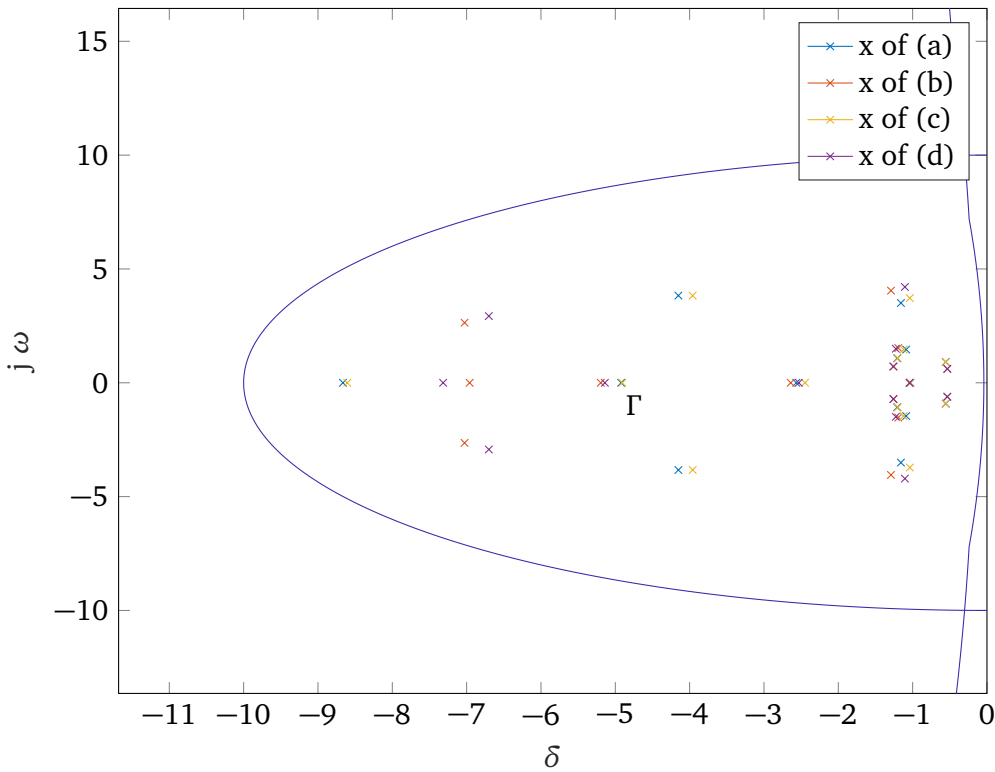
Figure 4.15.: Desired region of closed loop poles \Gamma and closed loop poles(x) of the four corner models
