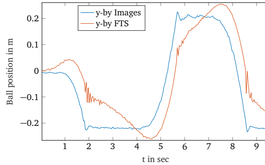
Figure 3.4.: Comparison of the BT algorithm with the method of (3.1) that utilizes torque measurements
